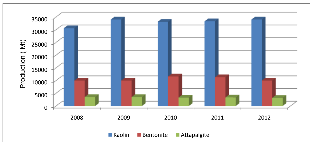
FIGURE 83: WORLD PRODUCTION OF SPECIAL CLAYS, 2012
