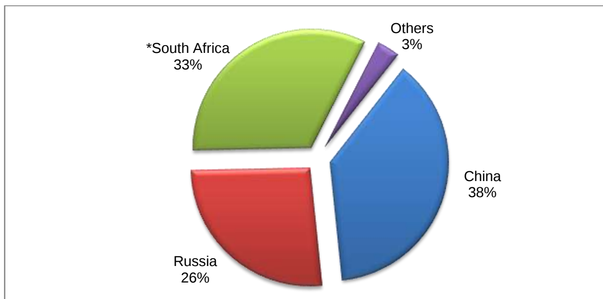
FIGURE 63: WORLD VANADIUM PRODUCTION, 2012
